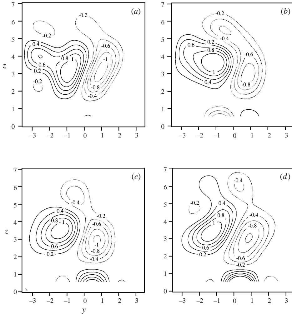
FIGURE 15. Spatial evolution of low-pass filtered \omega_x . (a) x = 4.5 , (b) x = 5.0 , (c) x = 5.5 , and (d) x = 6.0 . Contour intervals as marked. Dotted contours indicate negative values.
