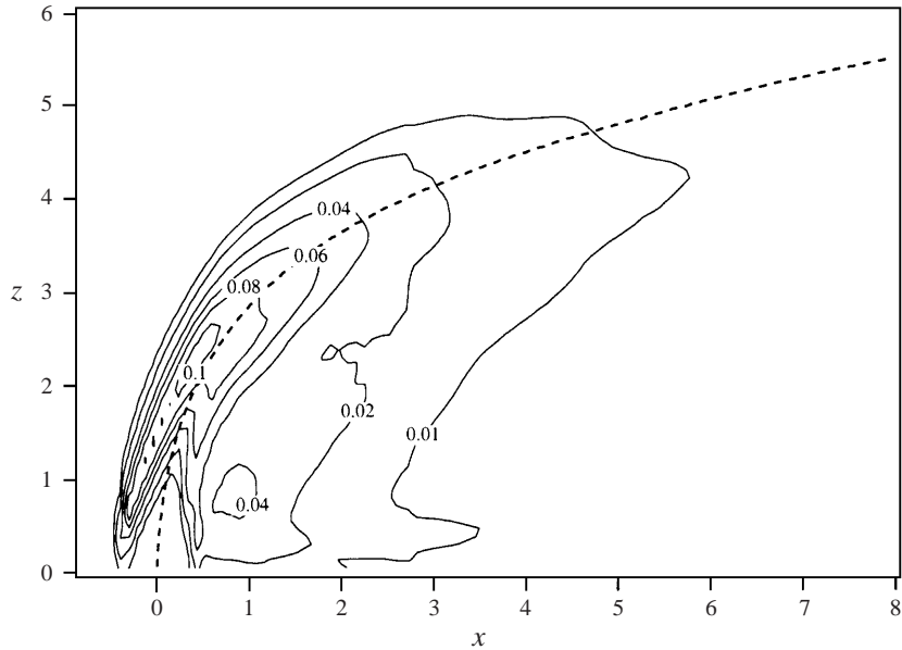
FIGURE 23. Contours of turbulent kinetic energy ( \langle q^2 \rangle / R^2 ) at the centreplane. Case 3II. Contour values as marked.
