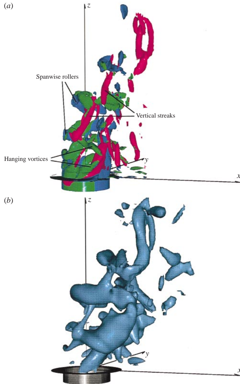
FIGURE 5. (a) Isosurfaces of vorticity. Green: \omega_x , blue: \omega_y , red: \omega_z . |\omega| = 20.0 . (b) Isosurfaces of pressure. \bar{p} = -1.8 .
